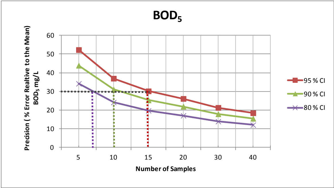
Figure 3-2. Relationship Between Precision (Estimated Error) and Sample Frequency for 95%, 90% and 80% Confidence Level
