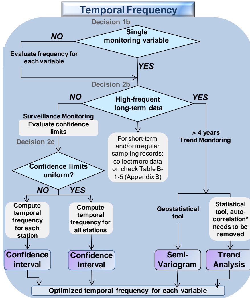
Figure 4-4. Decision-Making Flowchart to Optimize Temporal Frequency in a Water Quality Monitoring Network.
