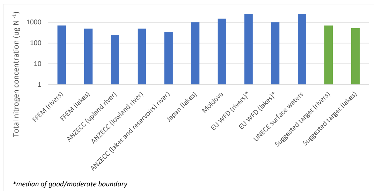
Figure 5: Examples of total nitrogen concentration targets used in countries (Source: data from multiple sources, refer to Annex 1)
